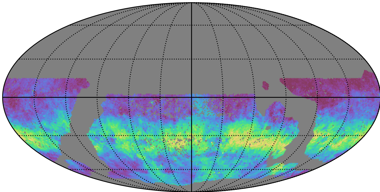
smc_lmc_v3.3_10yrs WFD u band: AngleRms rotSkyPos
