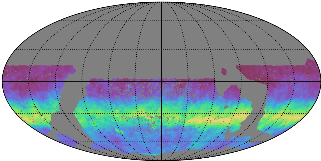
smc_lmc_v3.3_10yrs WFD r band: AngleRms rotSkyPos
