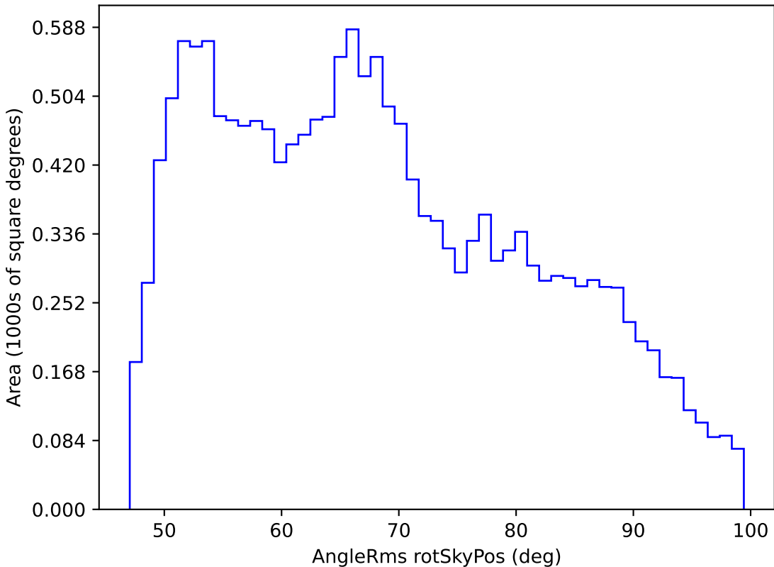
smc_lmc_v3.3_10yrs WFD r band: AngleRms rotSkyPos
