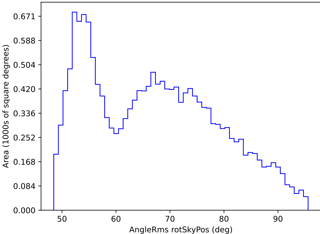
smc_lmc_v3.3_10yrs WFD i band: AngleRms rotSkyPos
