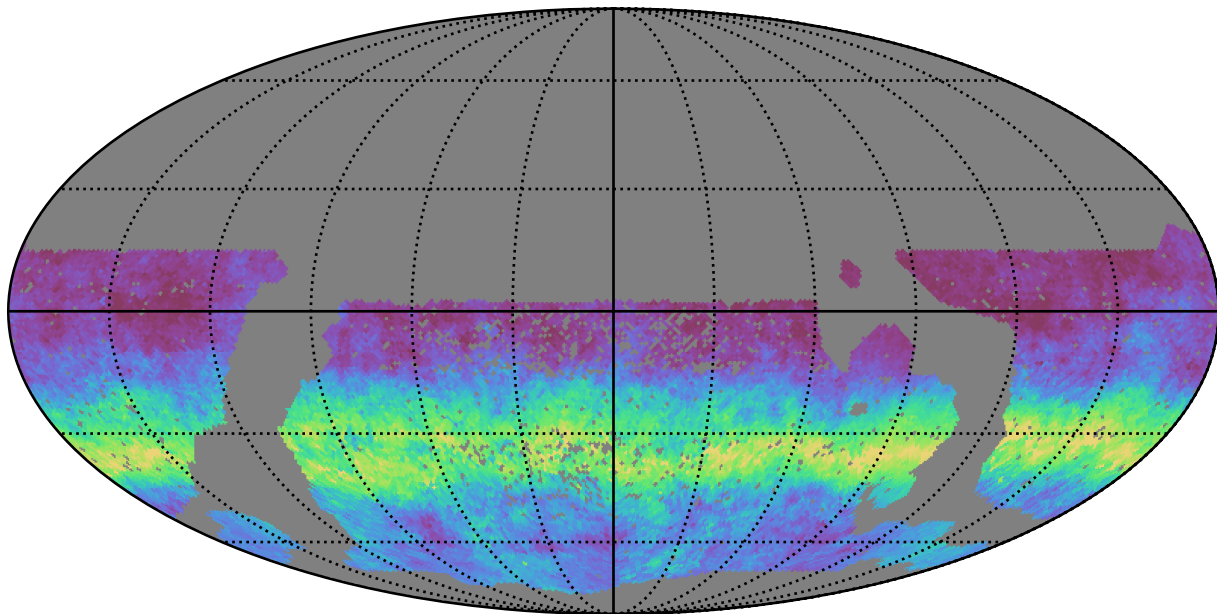
smc_lmc_v3.3_10yrs WFD g band: AngleRms rotSkyPos
