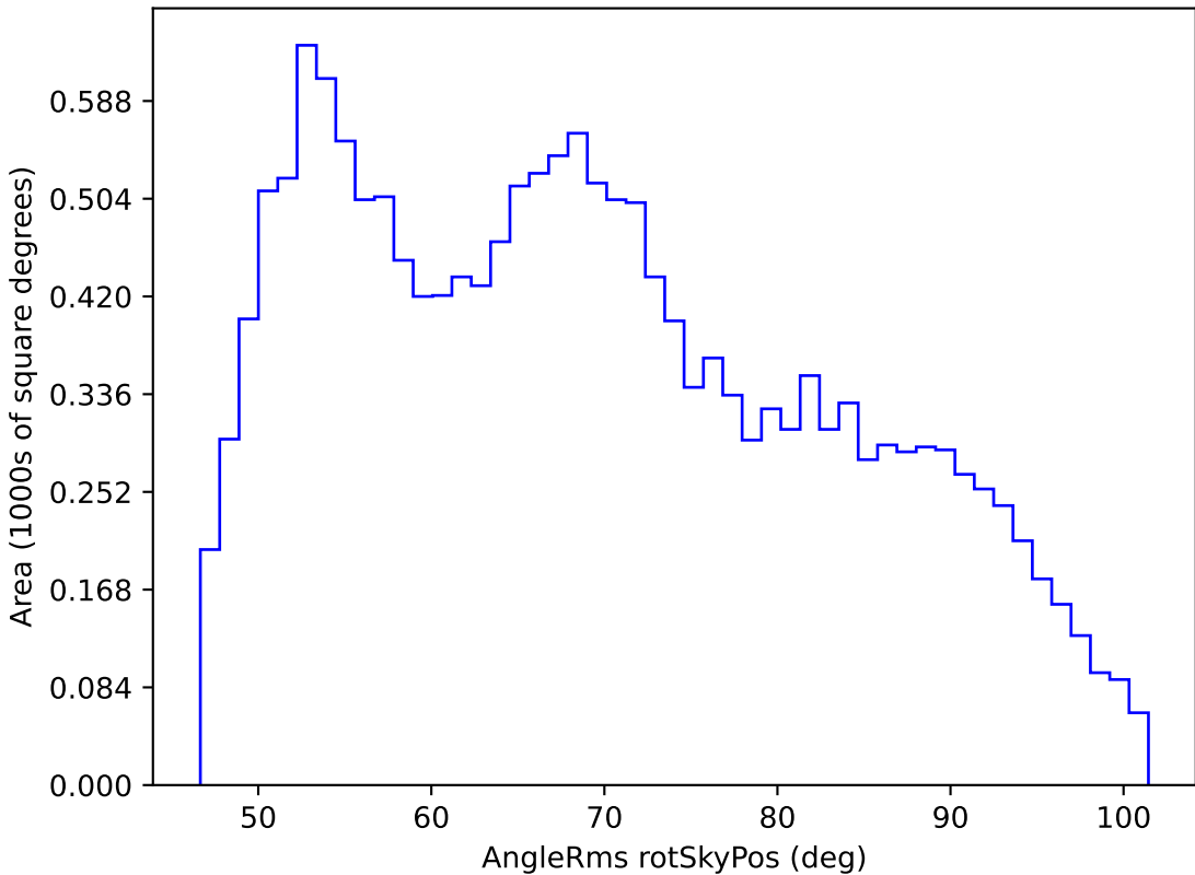
smc_lmc_v3.3_10yrs WFD g band: AngleRms rotSkyPos
