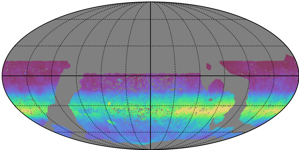
smc_lmc_v3.3_10yrs WFD all bands: AngleRms rotSkyPos
