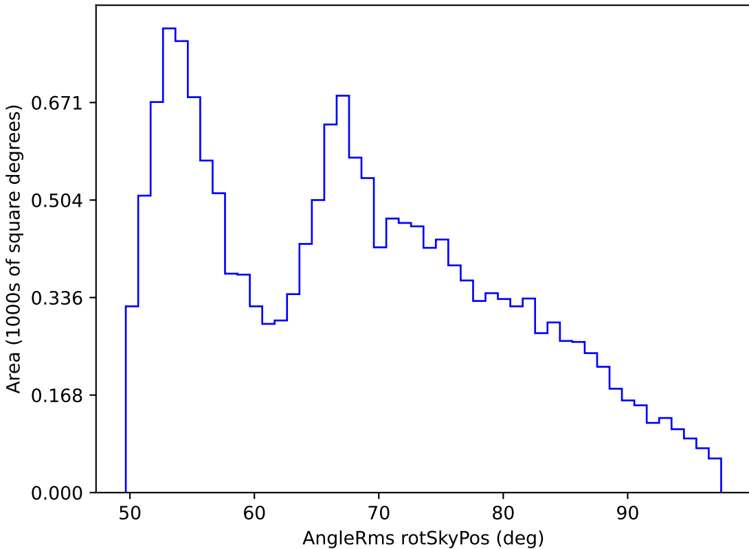
smc_lmc_v3.3_10yrs WFD all bands: AngleRms rotSkyPos
