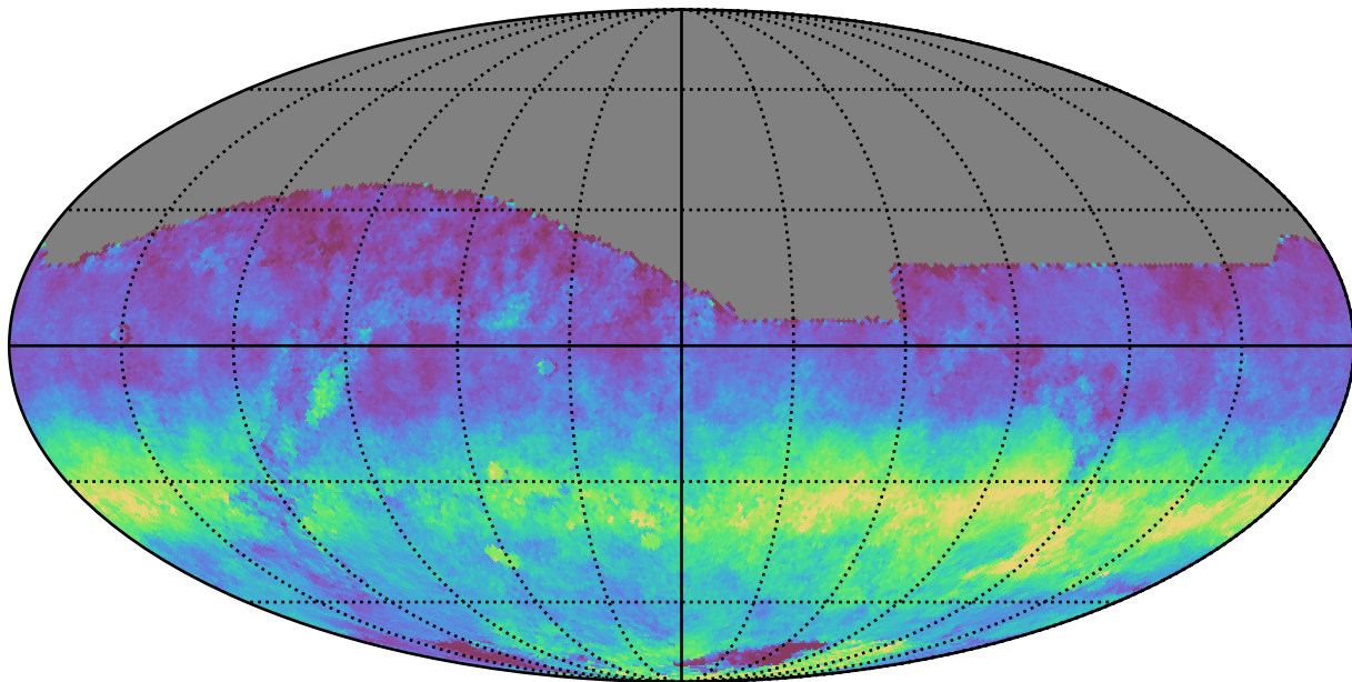
smc_lmc_v3.3_10yrs All sky z band: AngleRms rotSkyPos
