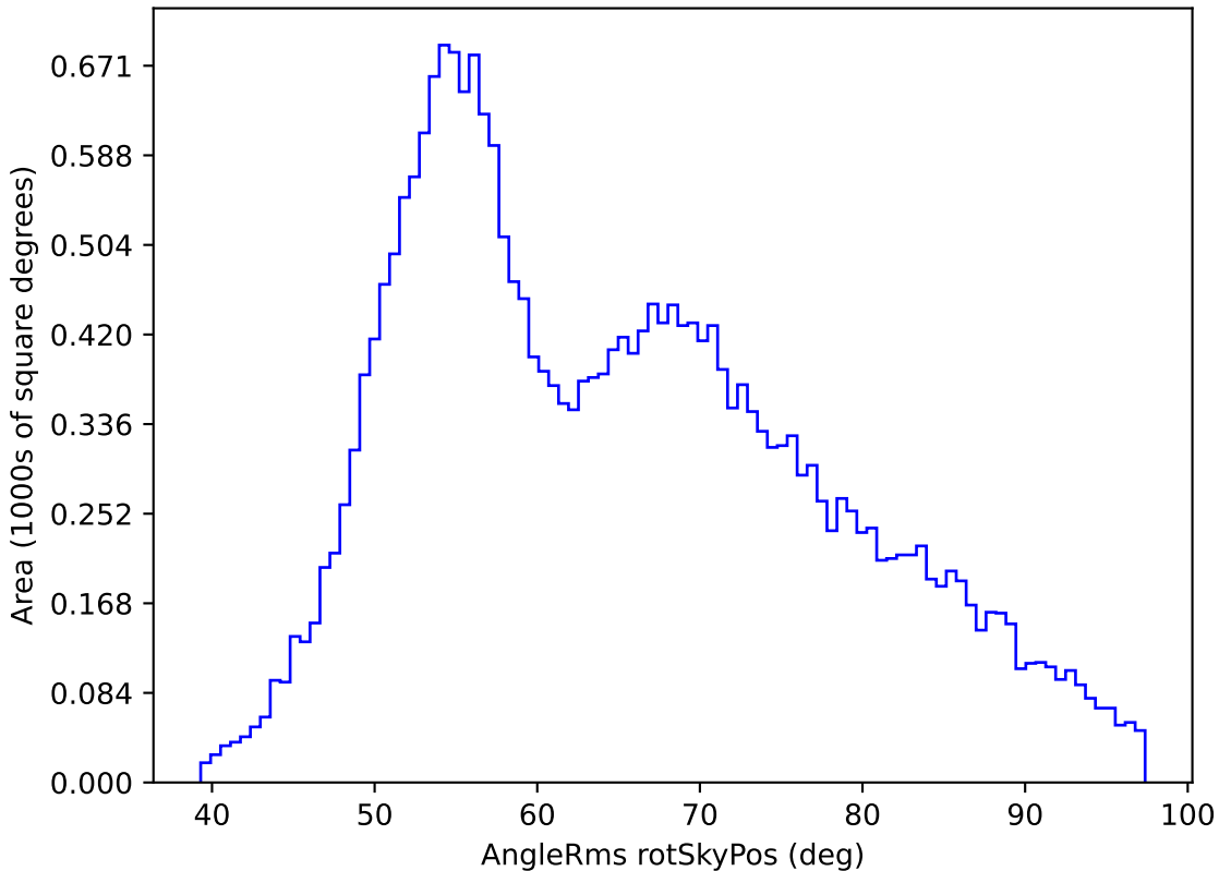
smc_lmc_v3.3_10yrs All sky z band: AngleRms rotSkyPos
