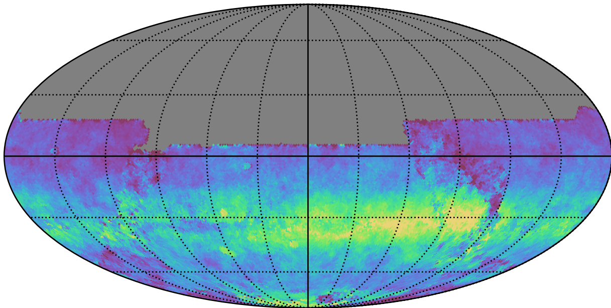
smc_lmc_v3.3_10yrs All sky y band: AngleRms rotSkyPos
