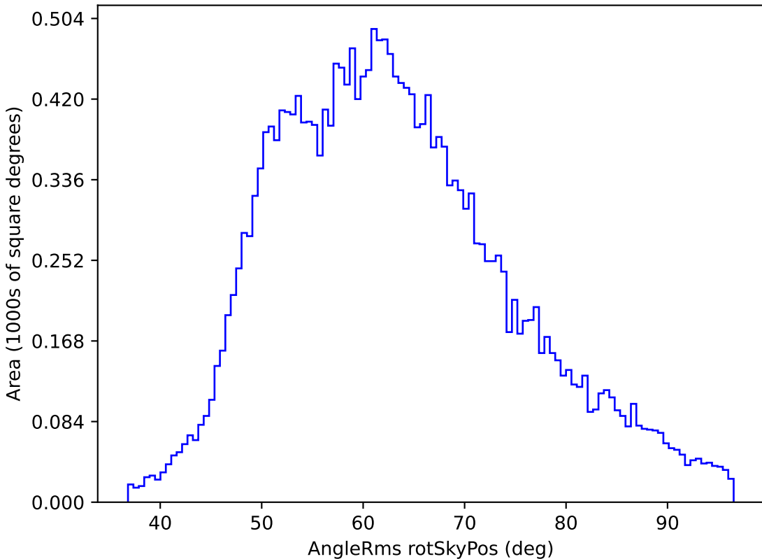
smc_lmc_v3.3_10yrs All sky y band: AngleRms rotSkyPos
