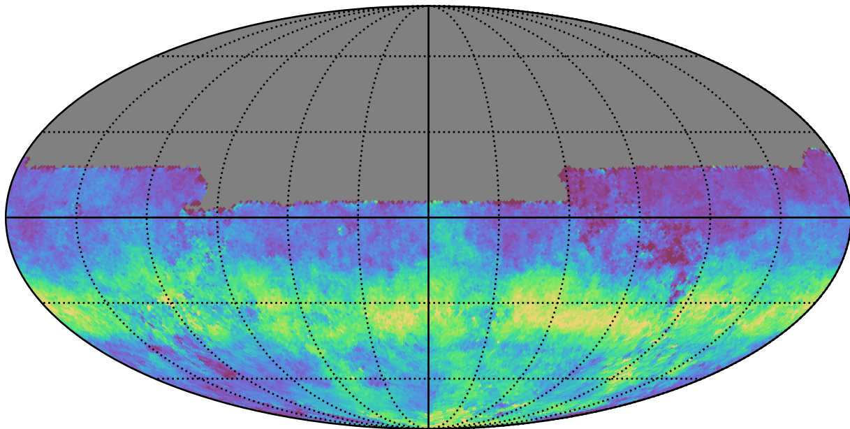
smc_lmc_v3.3_10yrs All sky u band: AngleRms rotSkyPos
