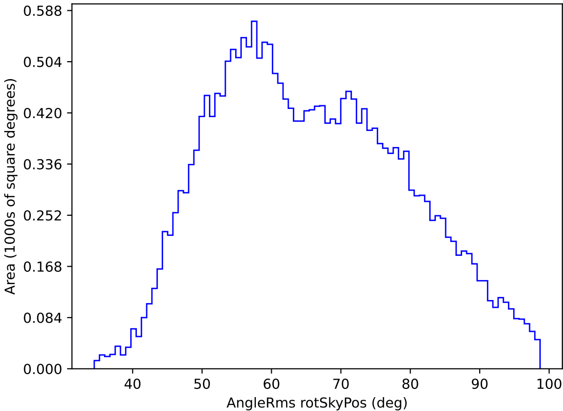
smc_lmc_v3.3_10yrs All sky u band: AngleRms rotSkyPos
