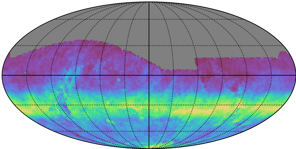
smc_lmc_v3.3_10yrs All sky r band: AngleRms rotSkyPos
