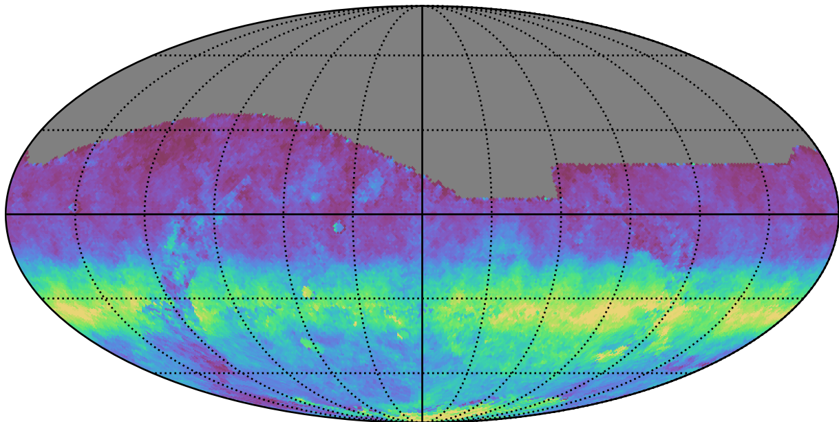
smc_lmc_v3.3_10yrs All sky i band: AngleRms rotSkyPos
