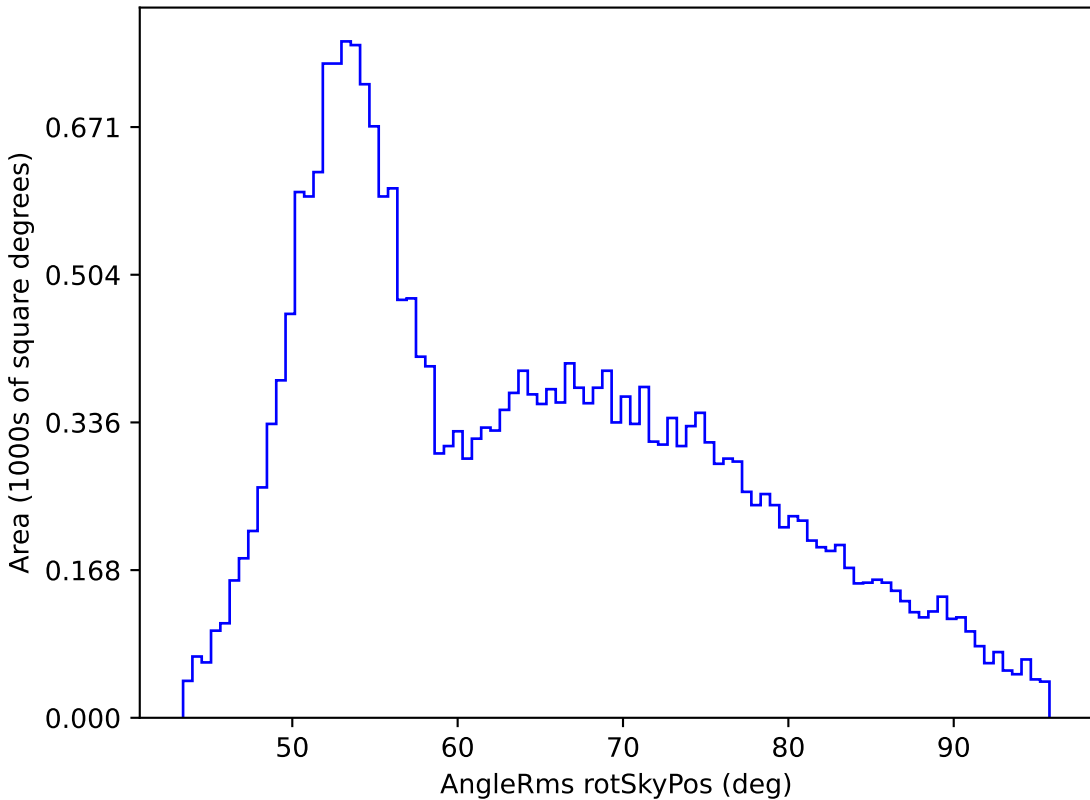
smc_lmc_v3.3_10yrs All sky i band: AngleRms rotSkyPos
