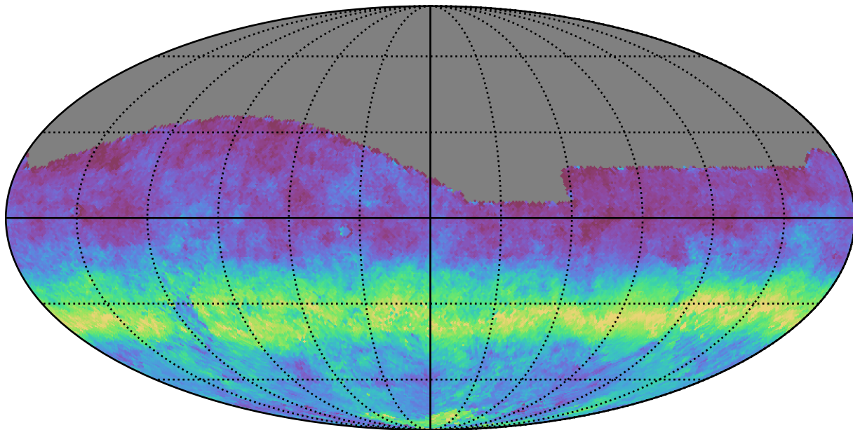
smc_lmc_v3.3_10yrs All sky g band: AngleRms rotSkyPos
