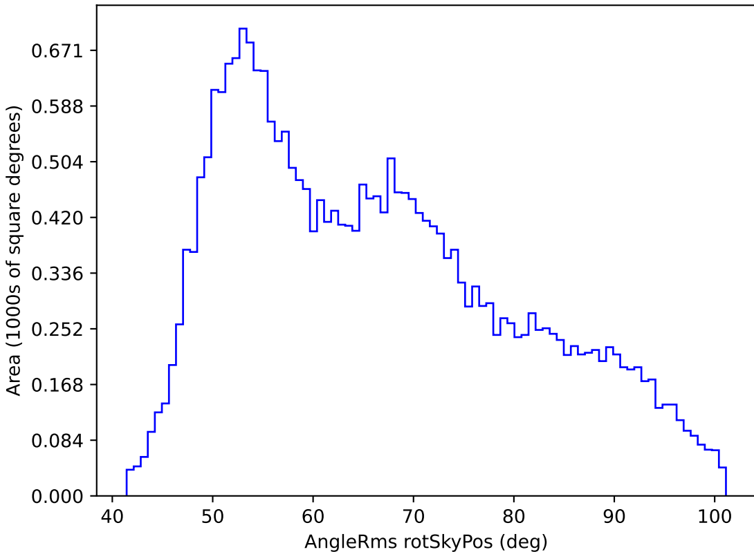
smc_lmc_v3.3_10yrs All sky g band: AngleRms rotSkyPos
