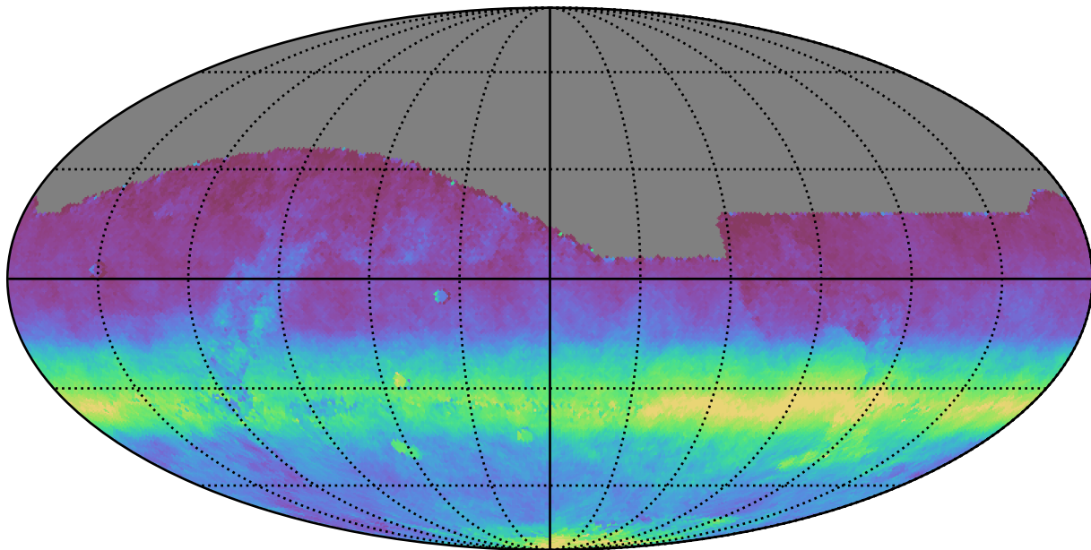
smc_lmc_v3.3_10yrs All sky all bands: AngleRms rotSkyPos
