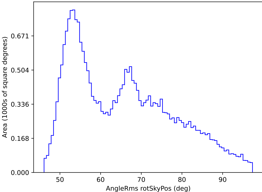
smc_lmc_v3.3_10yrs All sky all bands: AngleRms rotSkyPos
