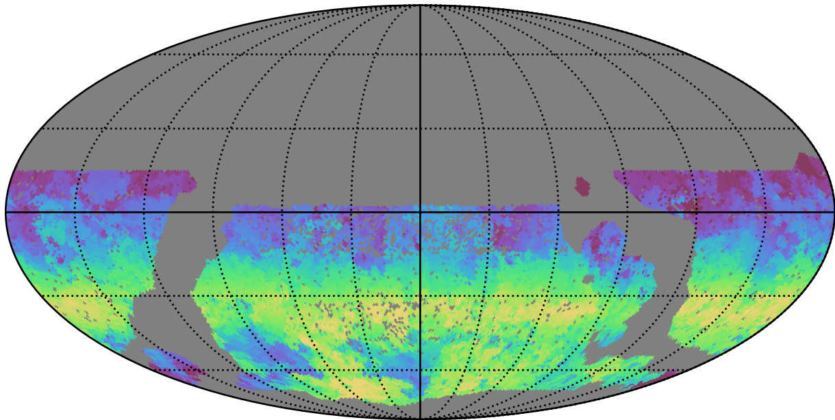
smc_lmc_v3.3_10yrs WFD u band: AngleRange rotSkyPos
