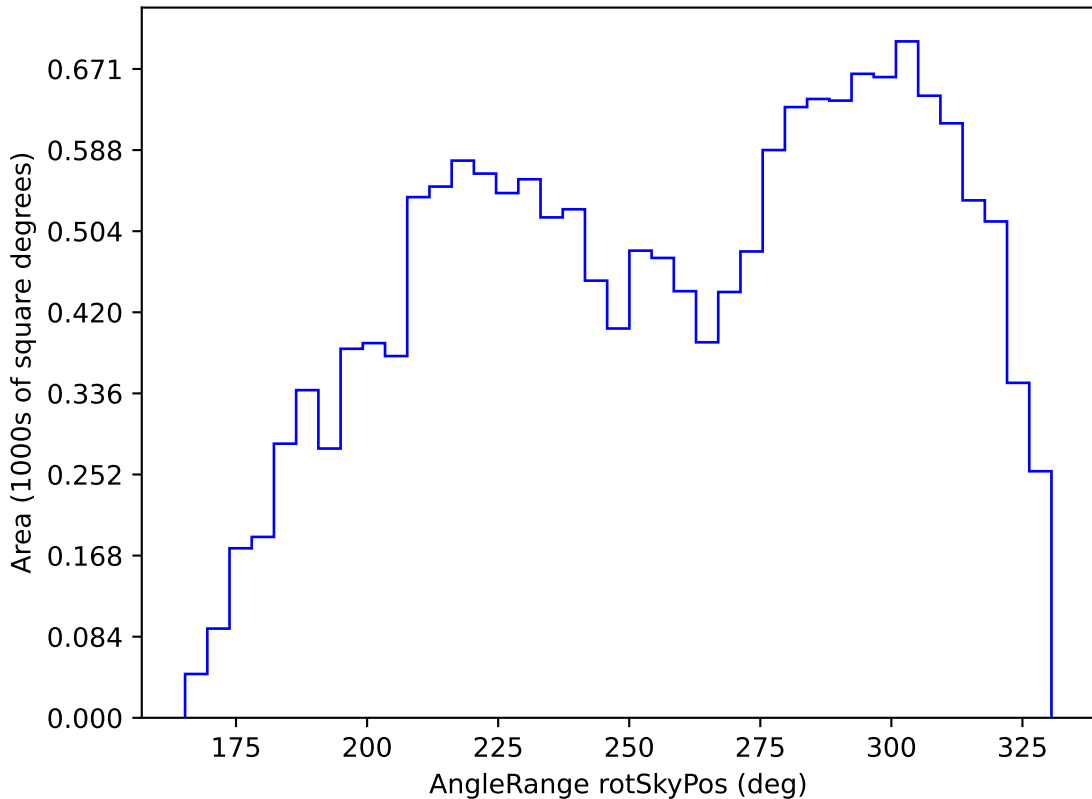
smc_lmc_v3.3_10yrs WFD u band: AngleRange rotSkyPos
