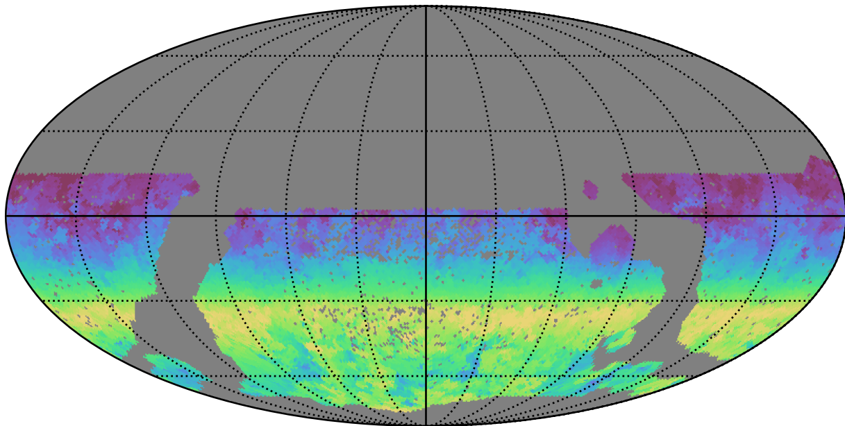
smc_lmc_v3.3_10yrs WFD r band: AngleRange rotSkyPos
