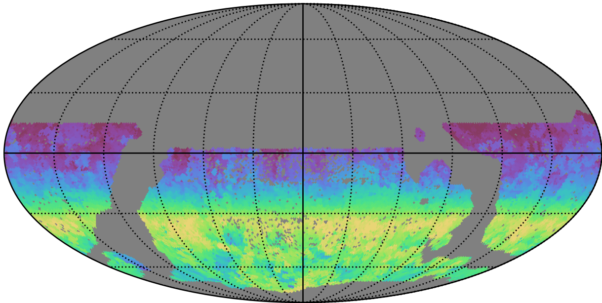
smc_lmc_v3.3_10yrs WFD i band: AngleRange rotSkyPos
