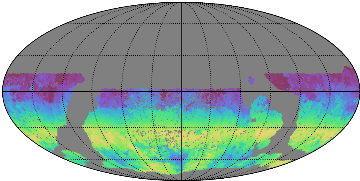
smc_lmc_v3.3_10yrs WFD g band: AngleRange rotSkyPos
