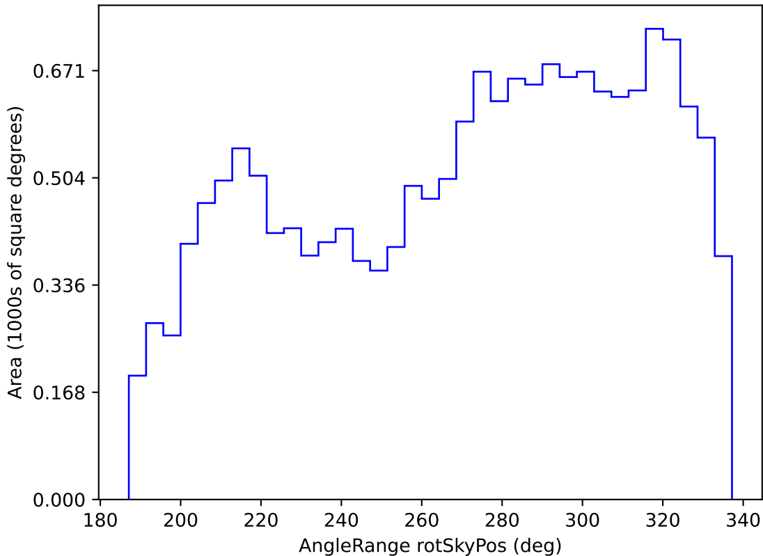
smc_lmc_v3.3_10yrs WFD g band: AngleRange rotSkyPos
