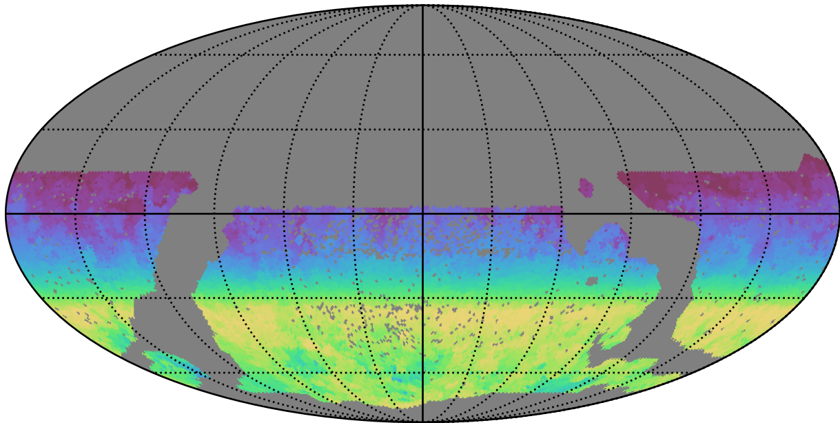
smc_lmc_v3.3_10yrs WFD all bands: AngleRange rotSkyPos
