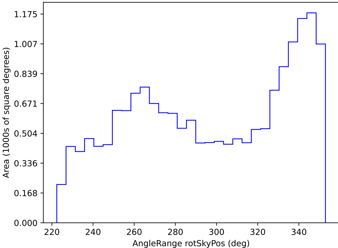
smc_lmc_v3.3_10yrs WFD all bands: AngleRange rotSkyPos
