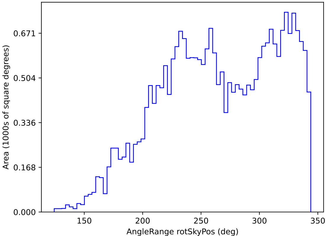
smc_lmc_v3.3_10yrs All sky z band: AngleRange rotSkyPos
