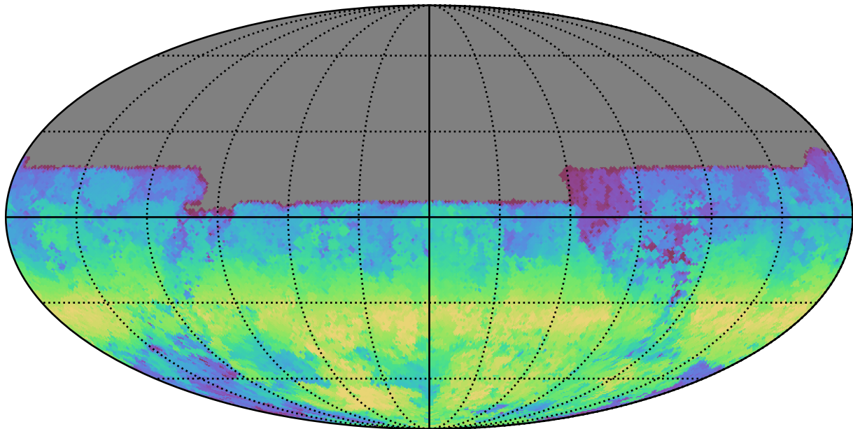
smc_lmc_v3.3_10yrs All sky u band: AngleRange rotSkyPos
