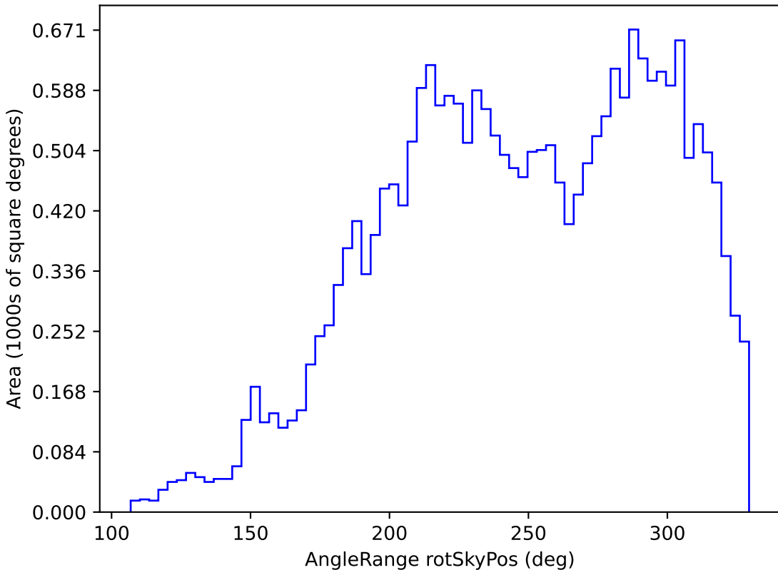
smc_lmc_v3.3_10yrs All sky u band: AngleRange rotSkyPos
