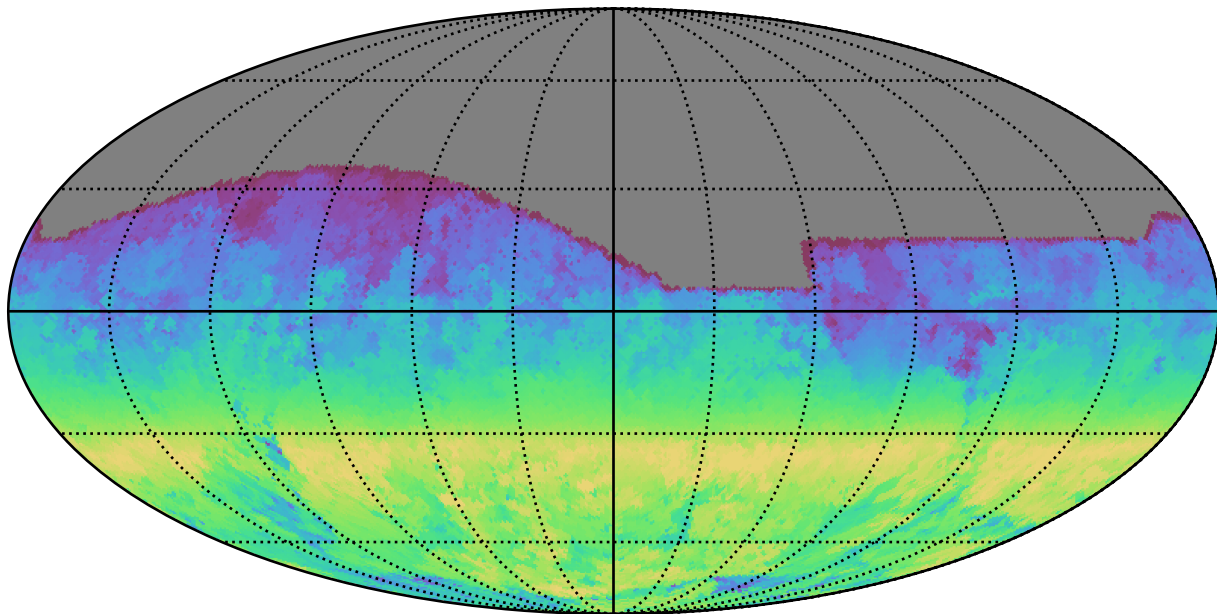
smc_lmc_v3.3_10yrs All sky r band: AngleRange rotSkyPos
