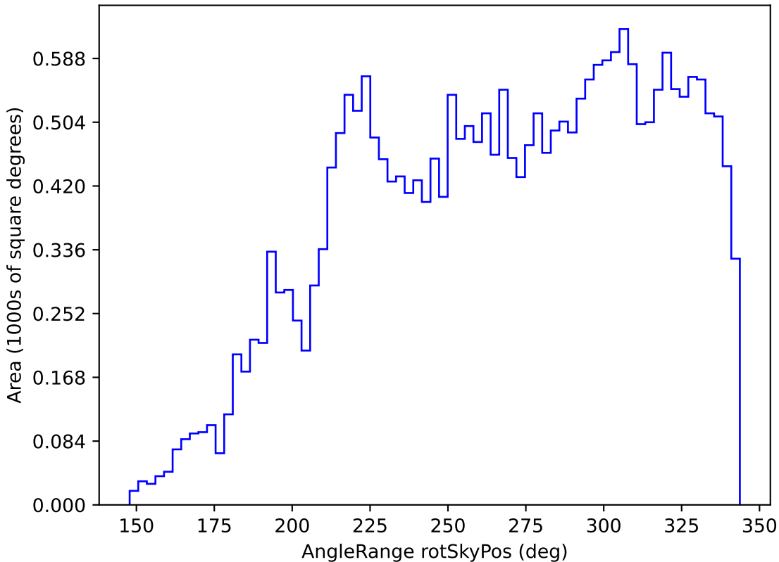
smc_lmc_v3.3_10yrs All sky r band: AngleRange rotSkyPos
