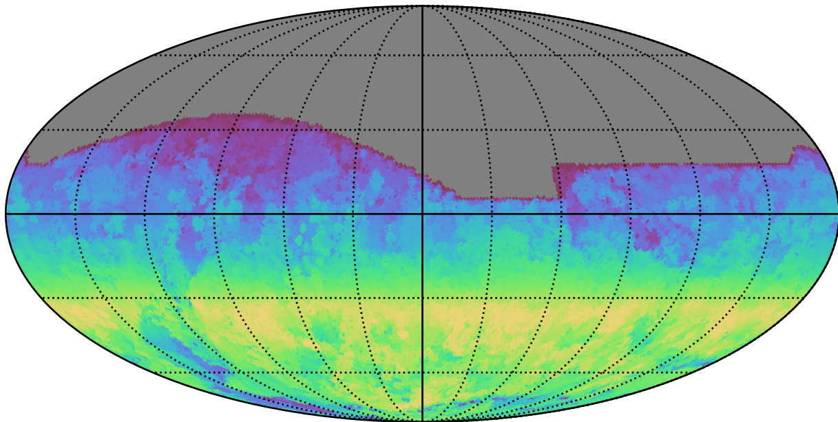
smc_lmc_v3.3_10yrs All sky i band: AngleRange rotSkyPos
