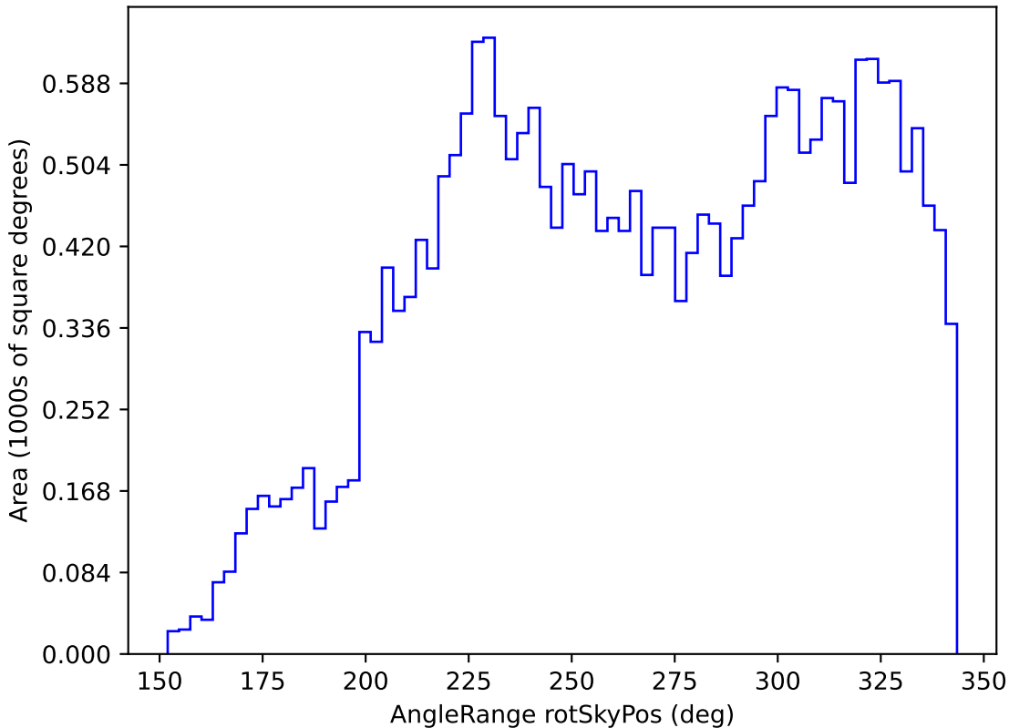
smc_lmc_v3.3_10yrs All sky i band: AngleRange rotSkyPos
