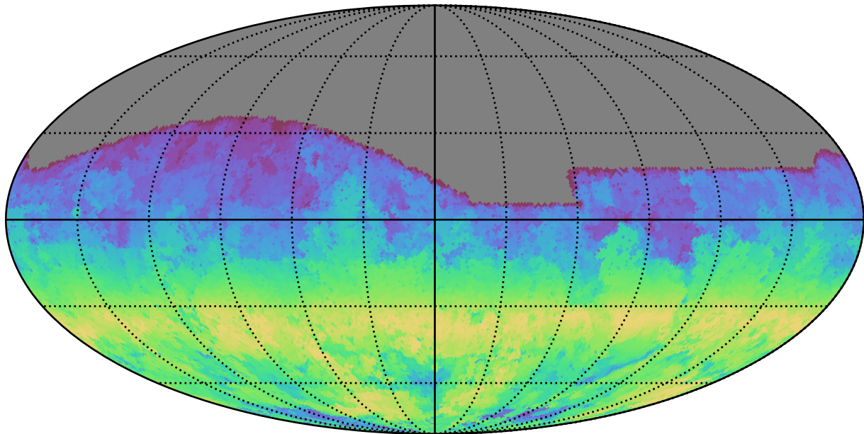
smc_lmc_v3.3_10yrs All sky g band: AngleRange rotSkyPos
