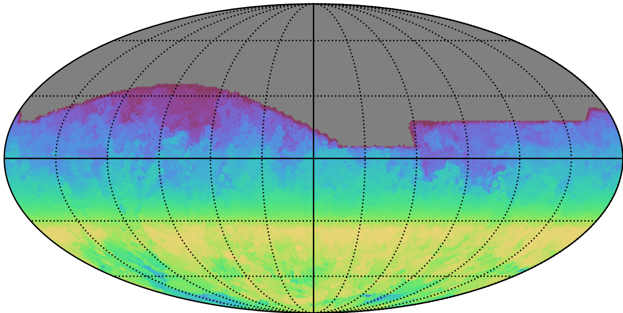
smc_lmc_v3.3_10yrs All sky all bands: AngleRange rotSkyPos
