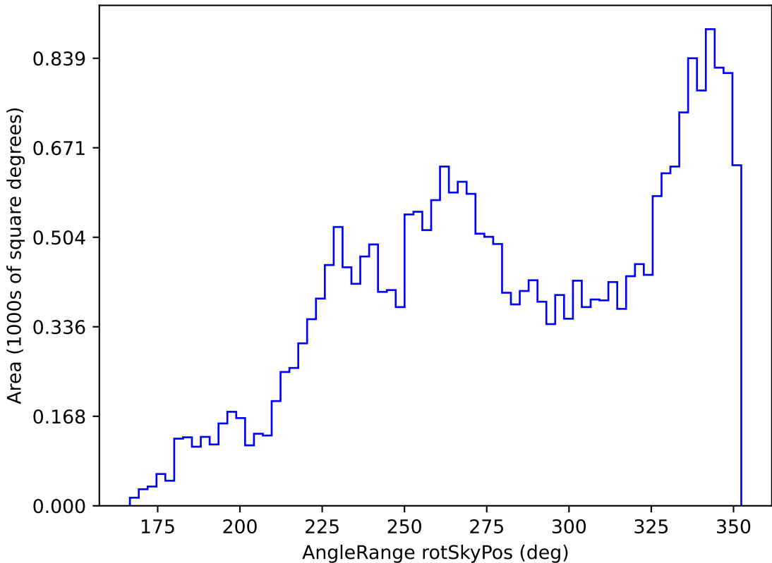
smc_lmc_v3.3_10yrs All sky all bands: AngleRange rotSkyPos
