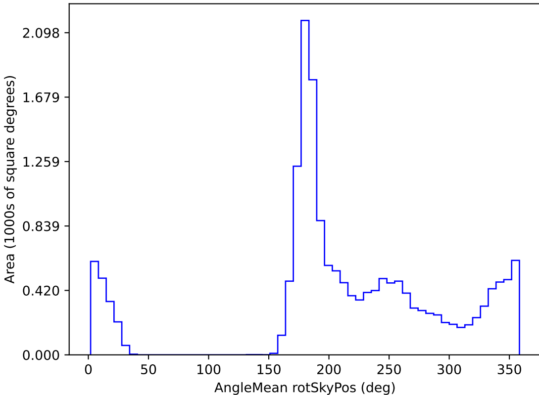
smc_lmc_v3.3_10yrs WFD z band: AngleMean rotSkyPos
