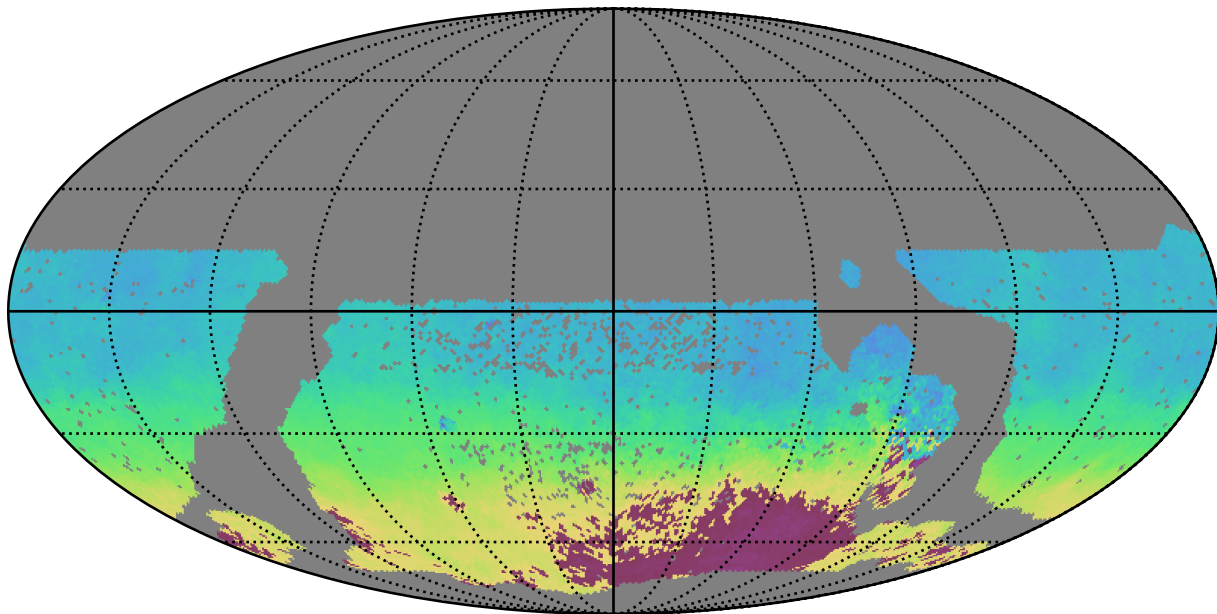
smc_lmc_v3.3_10yrs WFD y band: AngleMean rotSkyPos
