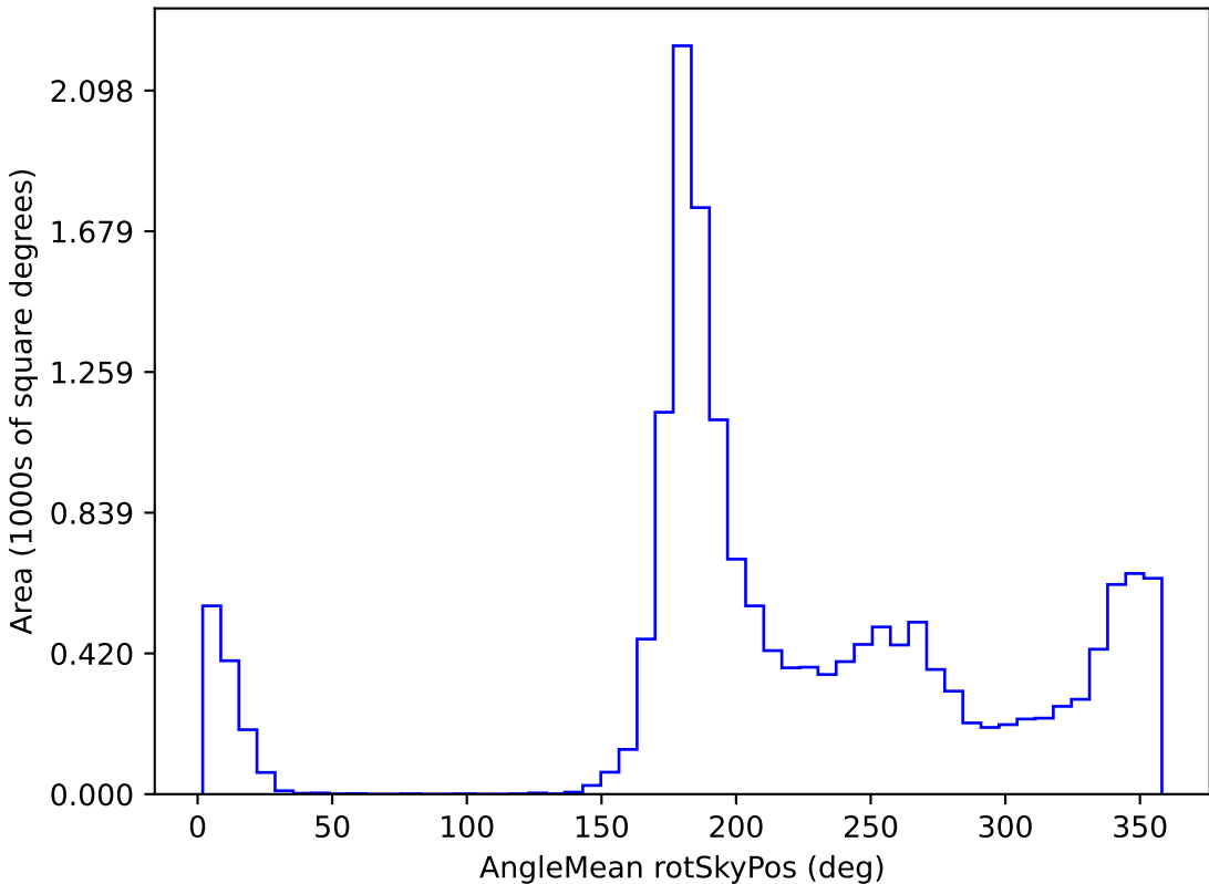
smc_lmc_v3.3_10yrs WFD y band: AngleMean rotSkyPos
