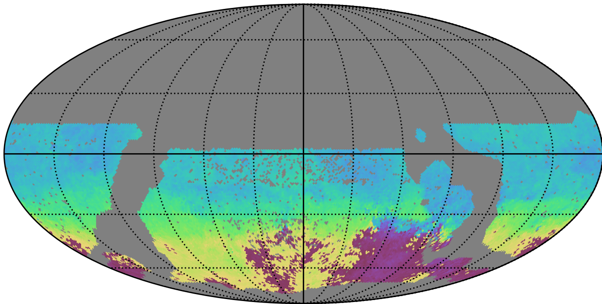
smc_lmc_v3.3_10yrs WFD u band: AngleMean rotSkyPos
