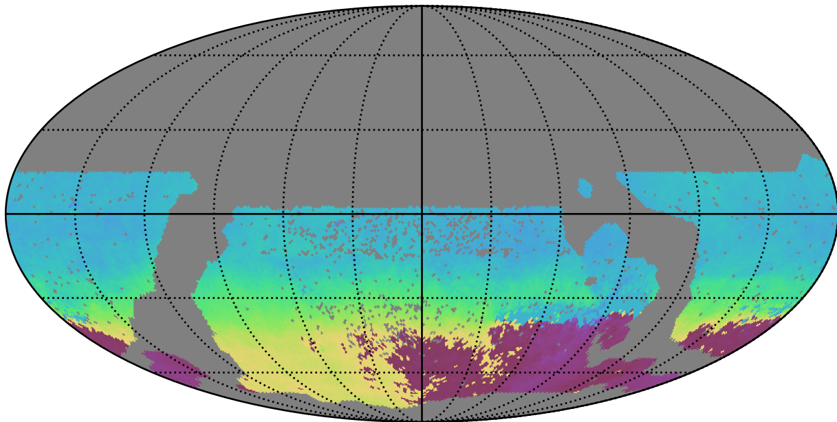
smc_lmc_v3.3_10yrs WFD r band: AngleMean rotSkyPos
