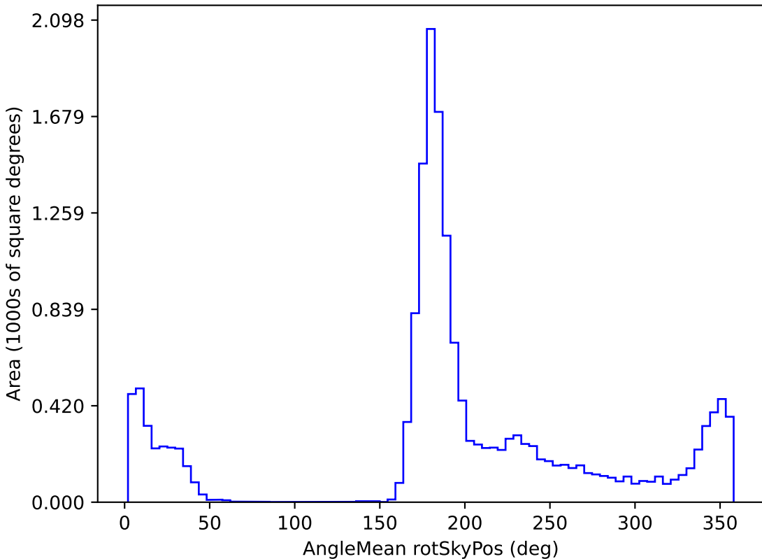
smc_lmc_v3.3_10yrs WFD r band: AngleMean rotSkyPos
