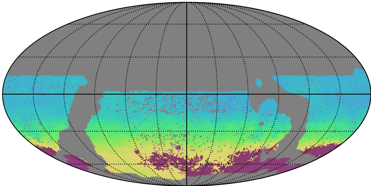
smc_lmc_v3.3_10yrs WFD i band: AngleMean rotSkyPos
