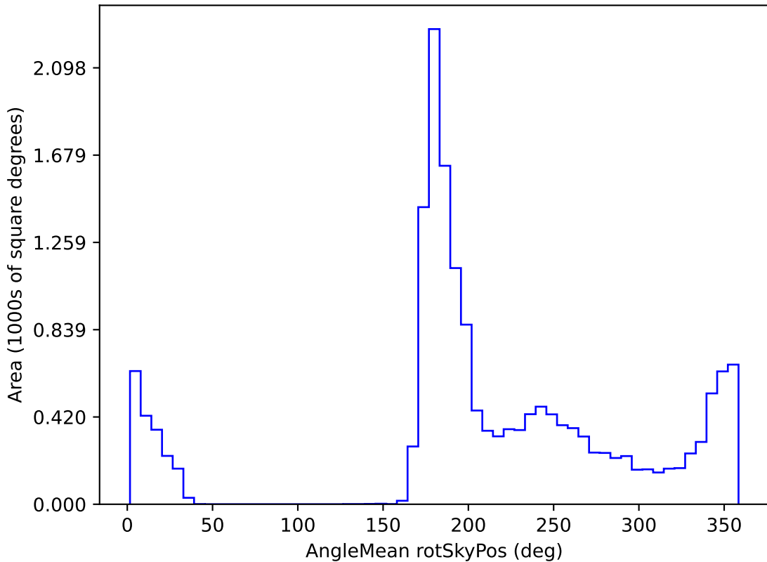
smc_lmc_v3.3_10yrs WFD i band: AngleMean rotSkyPos
