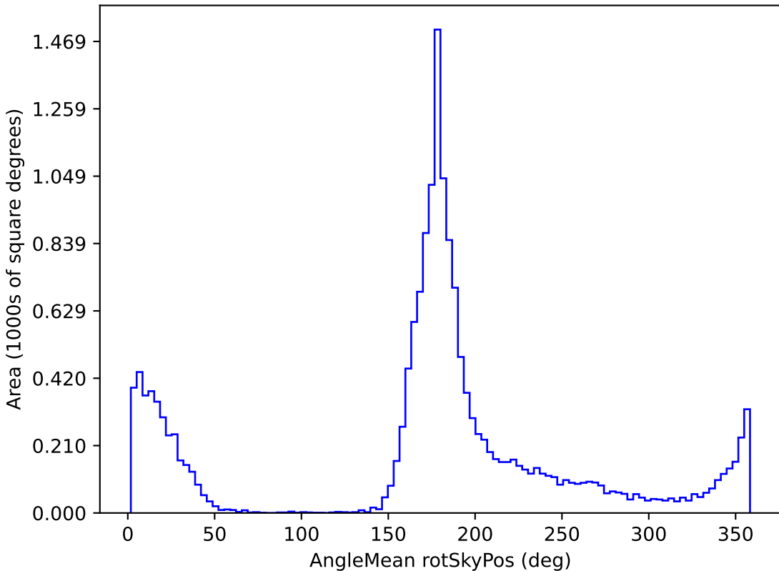
smc_lmc_v3.3_10yrs WFD g band: AngleMean rotSkyPos
