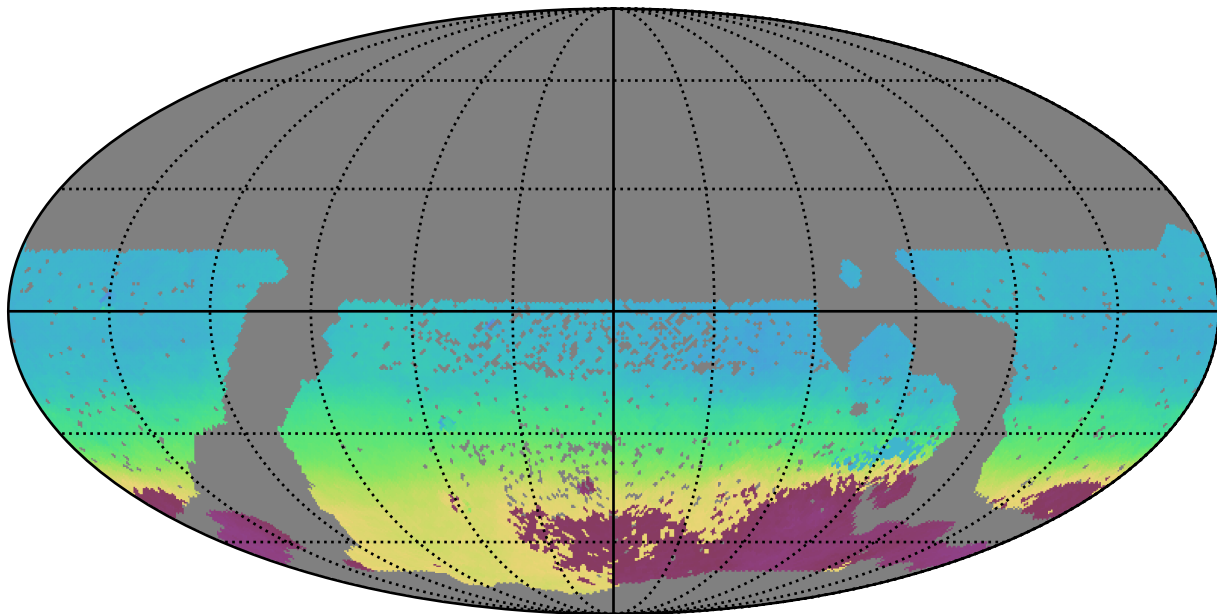
smc_lmc_v3.3_10yrs WFD all bands: AngleMean rotSkyPos
