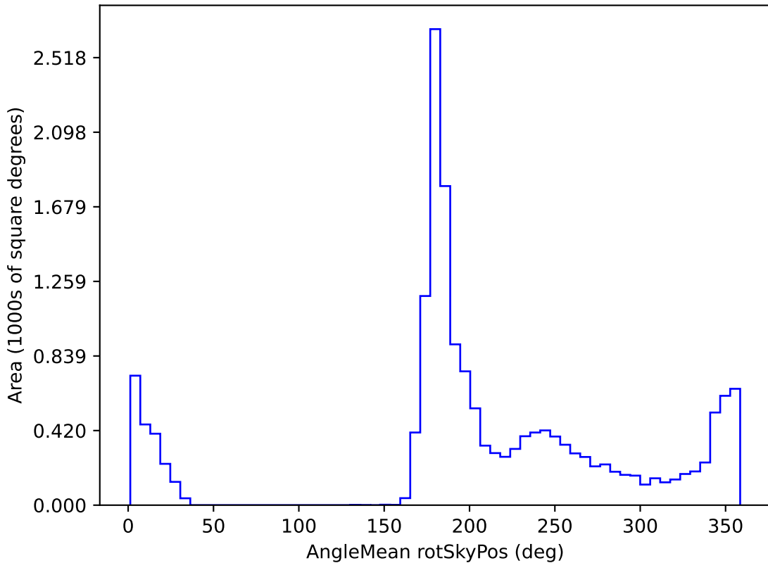
smc_lmc_v3.3_10yrs WFD all bands: AngleMean rotSkyPos
